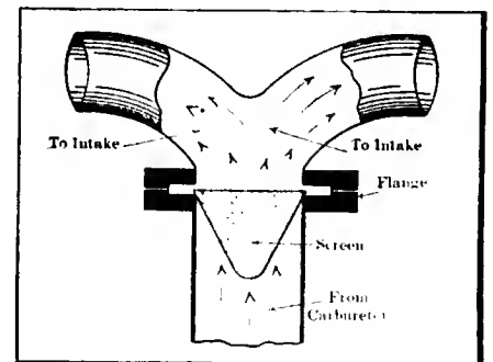
Fig. 4—Showing indentation in flanges so as to form a place for the supporting flange of the screen in the intake manifold
